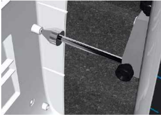
Measuring centre distances on a plastic casing of an electronic box
